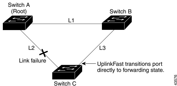
Figure 22-4 UplinkFast Example After Direct Link Failure
