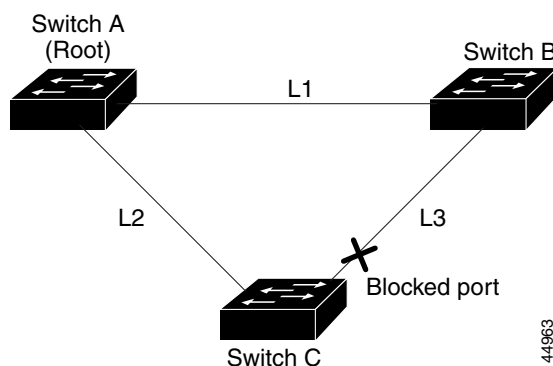
Figure 22-6 BackboneFast Example Before Indirect Link Failure
