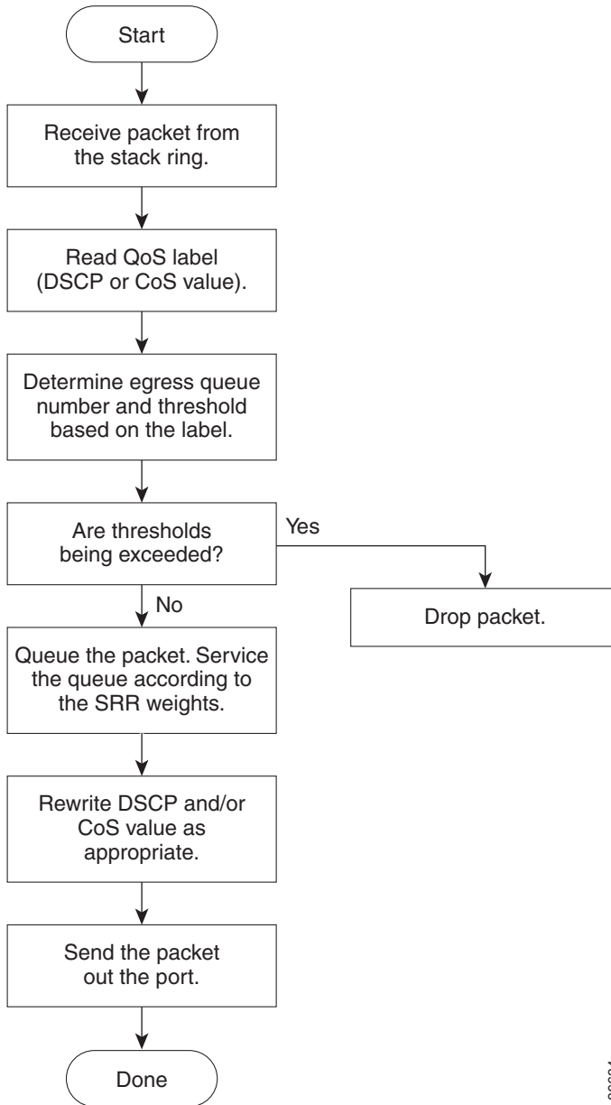
Figure 1-9 Queueing and Scheduling Flowchart for Egress Ports
