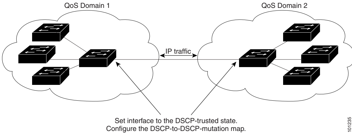
Figure 1-12 DSCP-Trusted State on a Port Bordering Another QoS Domain
