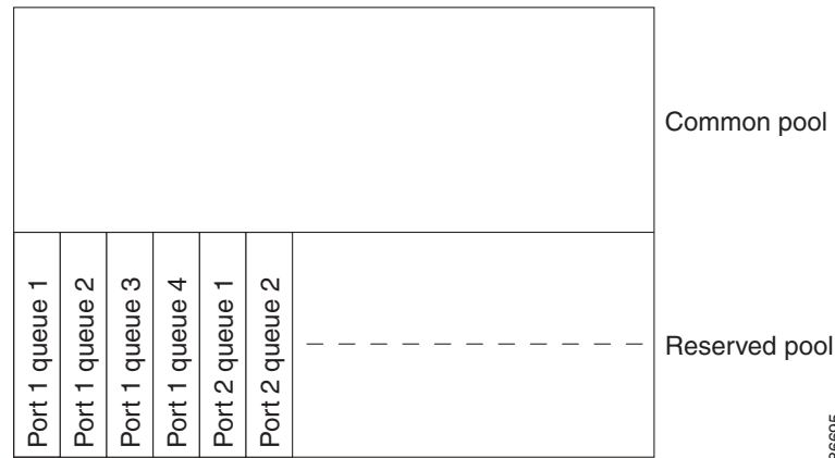
Figure 1-10 Egress Queue Buffer Allocation
