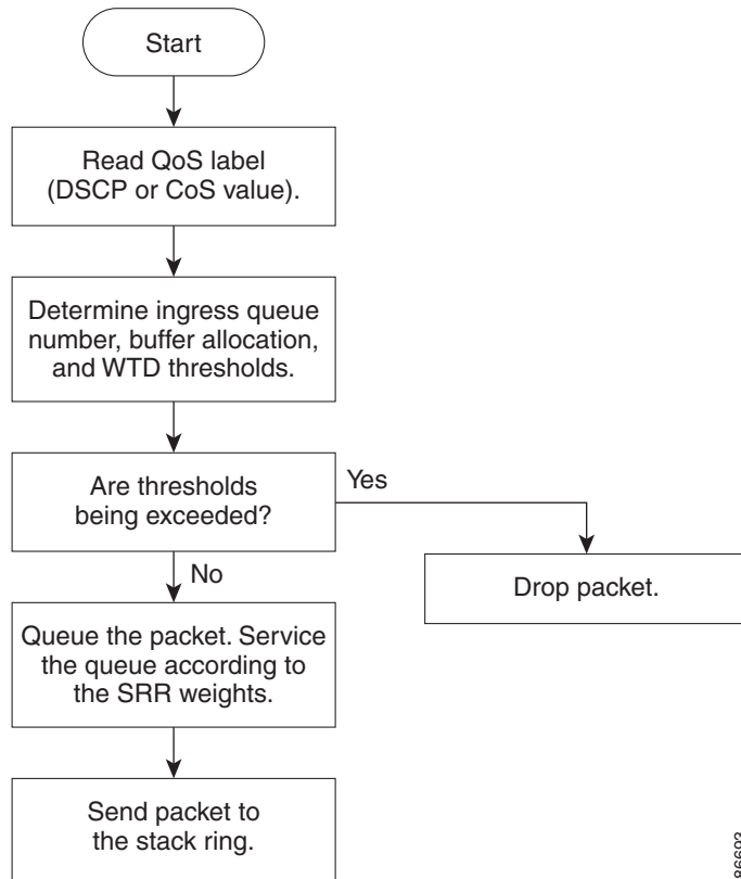
Figure 1-8 Queueing and Scheduling Flowchart for Ingress Ports
