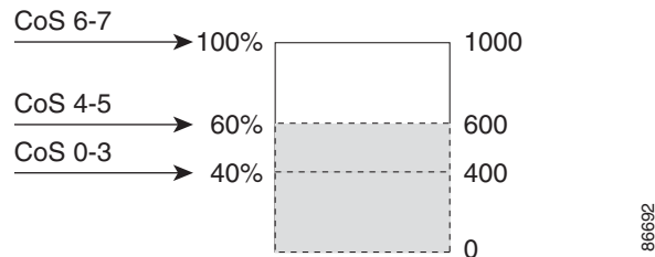
Figure 1-7 WTD and Queue Operation
