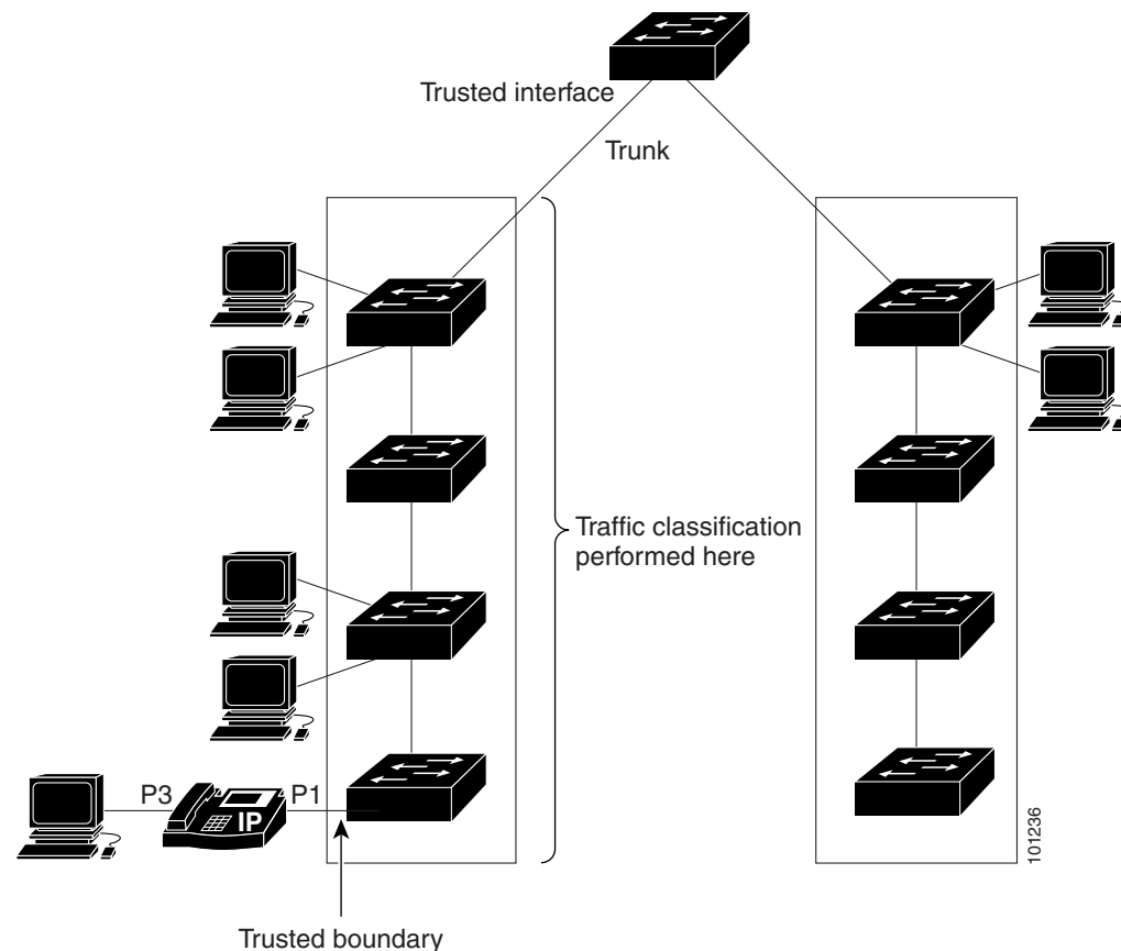
Figure 1-11 Port Trusted States Within the QoS Domain
