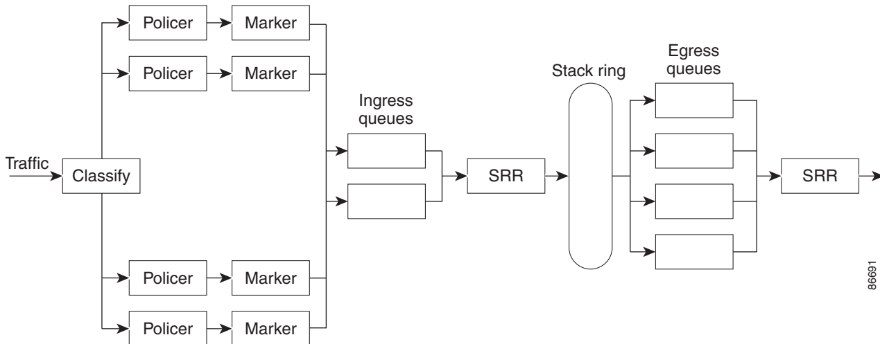
Figure 1-6 Ingress and Egress Queue Location
