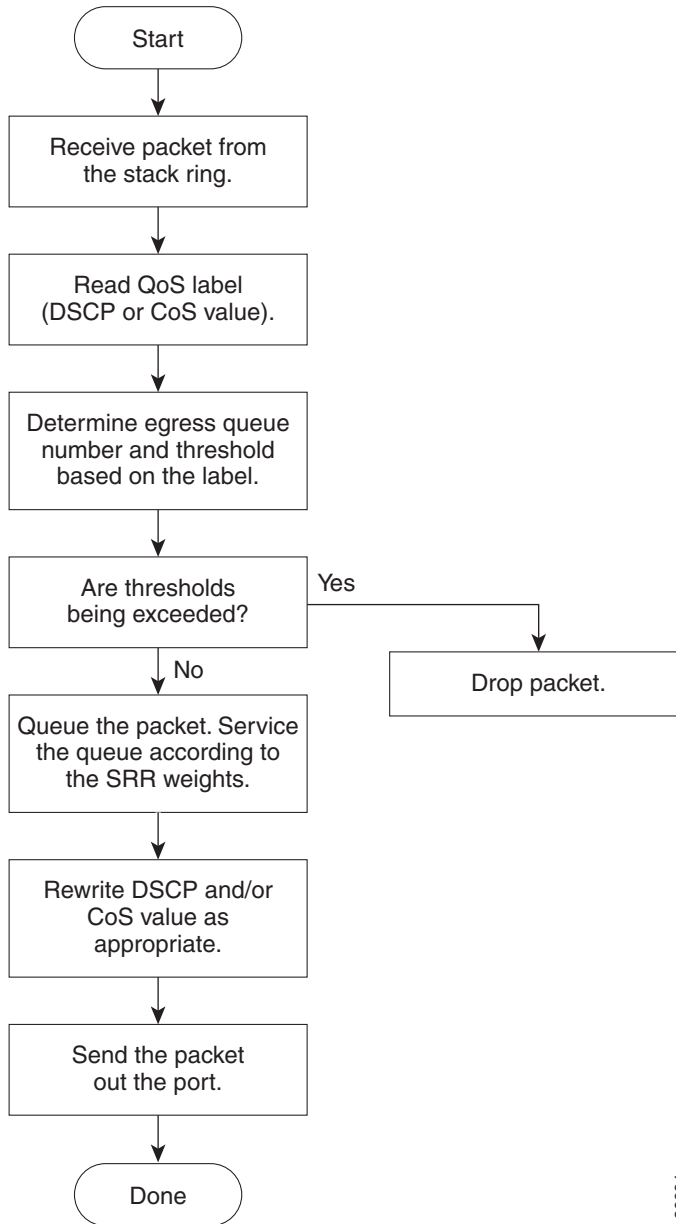
Figure 35-9 Queueing and Scheduling Flowchart for Egress Ports
