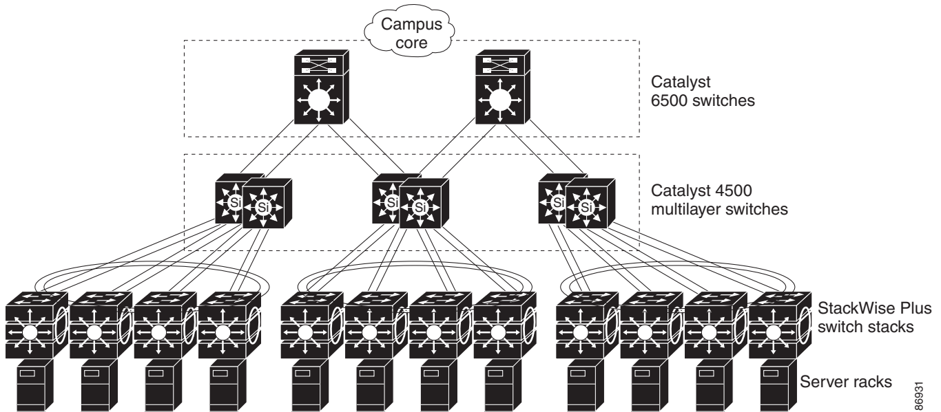
Figure 1-4 Server Aggregation
