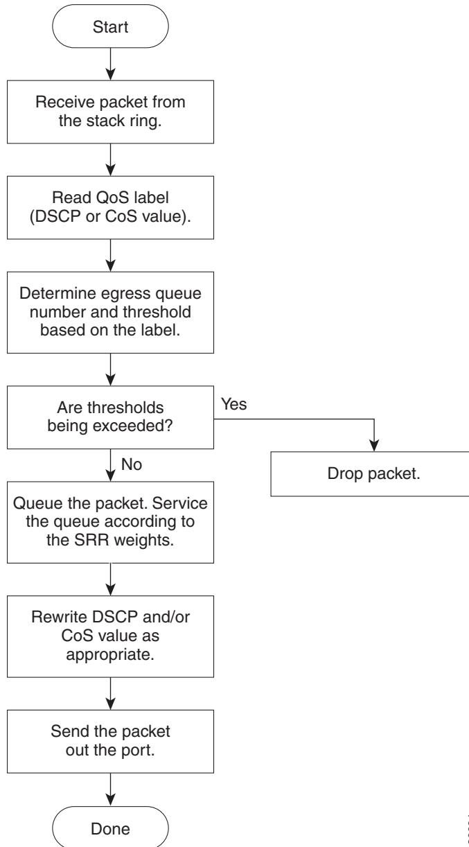
Figure 36-9 Queueing and Scheduling Flowchart for Egress Ports
