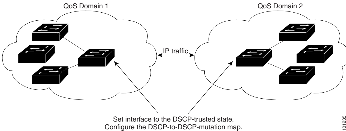
Figure 36-13 DSCP-Trusted State on a Port Bordering Another QoS Domain
