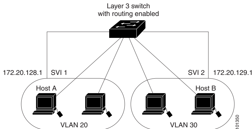
Figure 12-1 Connecting VLANs with the Catalyst 3750 Switch
