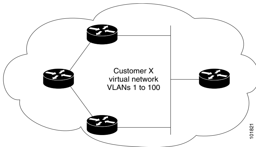
Figure 17-5 Layer 2 Network Topology without Proper Convergence
