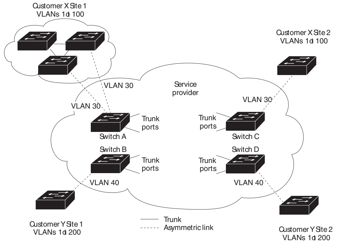
Figure 17-4 Layer 2 Protocol Tunneling
