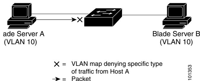
Figure 32-2 Using VLAN Maps to Control Traffic
