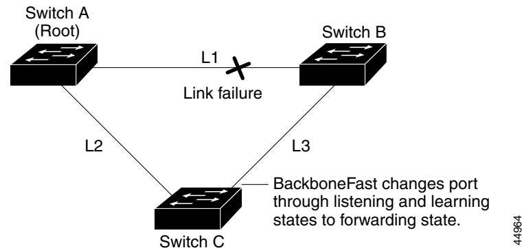
Figure 19-7 BackboneFast Example After Indirect Link Failure
