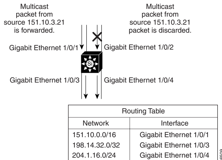
Figure 31-2 RPF Check
