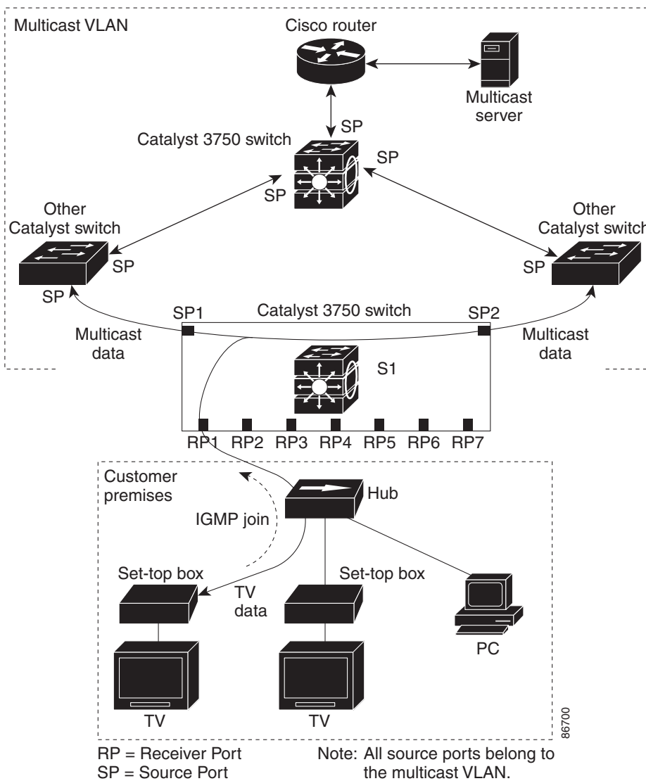
Figure 15-3 Multicast VLAN Registration Example
