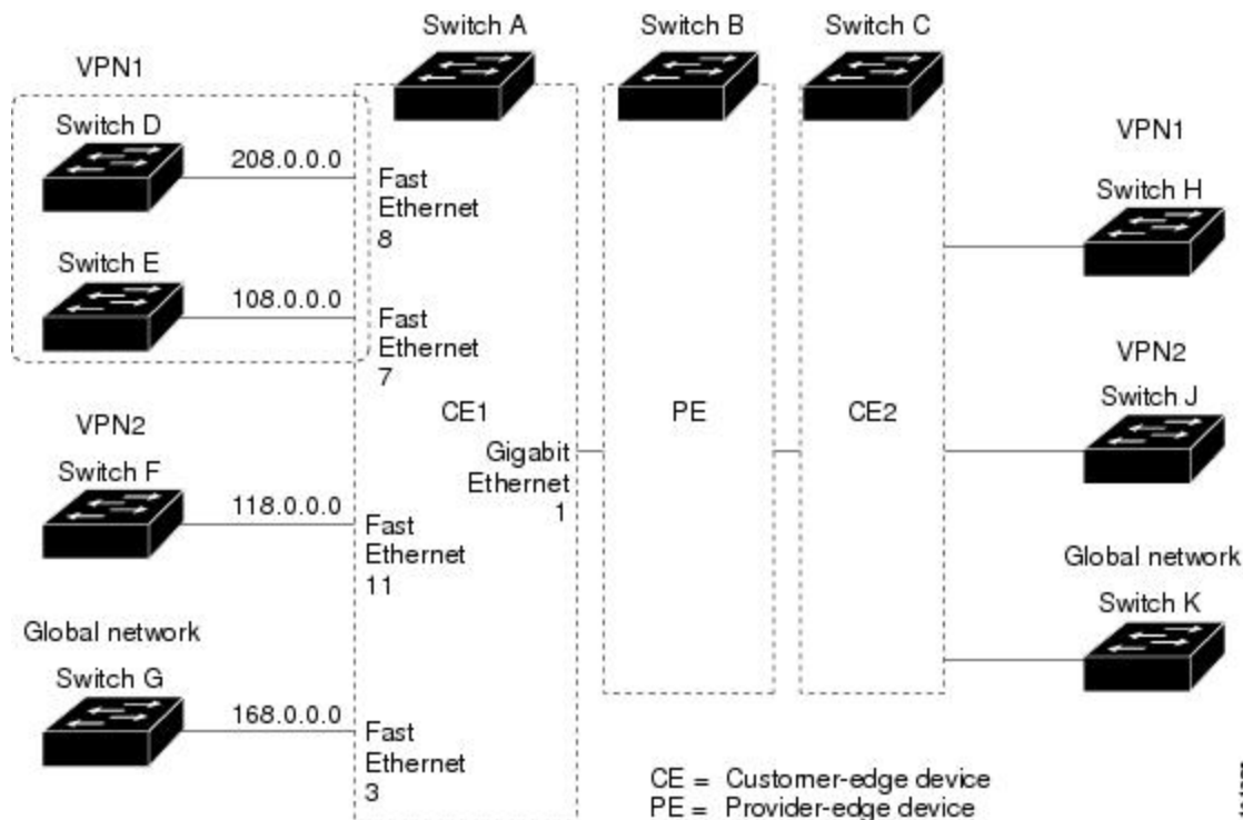
Figure 7: Multi-VRF CE Configuration Example
