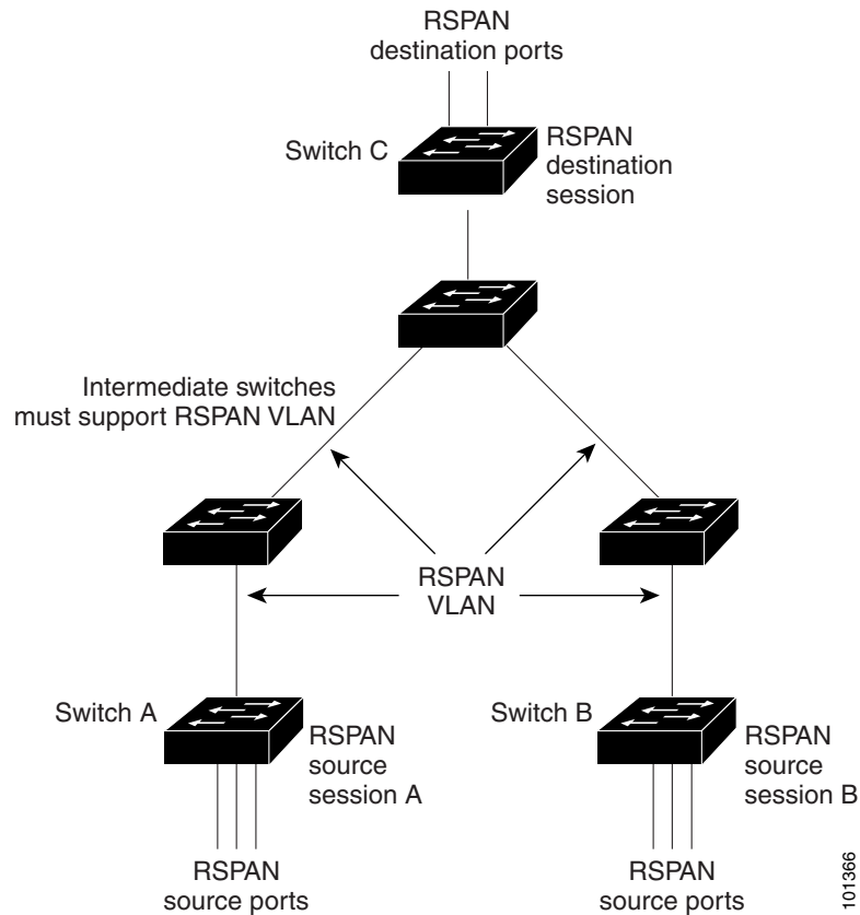
Figure 32-2 Example of RSPAN Configuration
