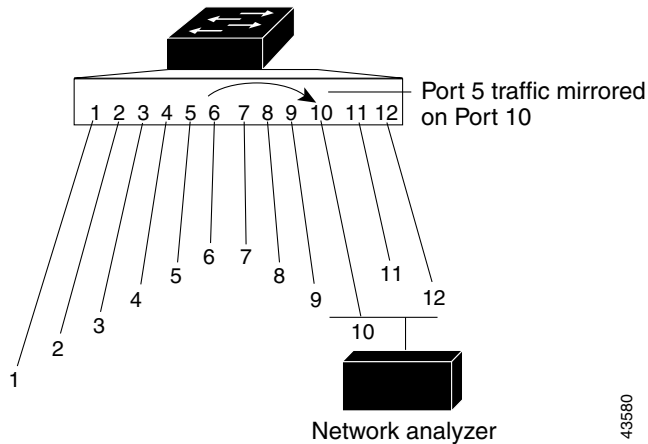
Figure 32-1 Example of Local SPAN Configuration on a Single Switch
