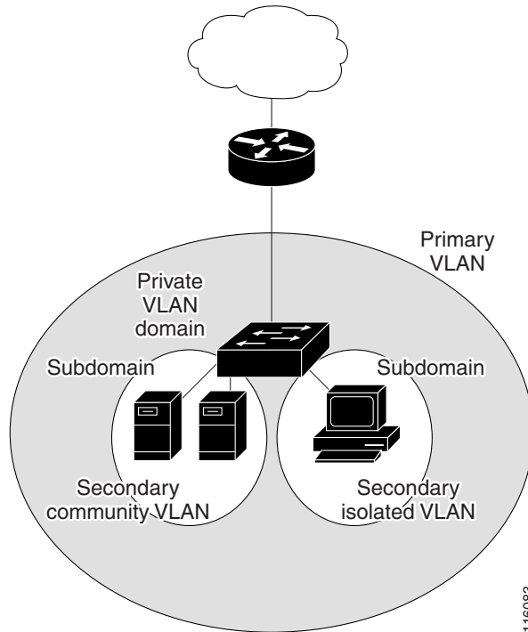
Figure 18-1 Private-VLAN Domain
