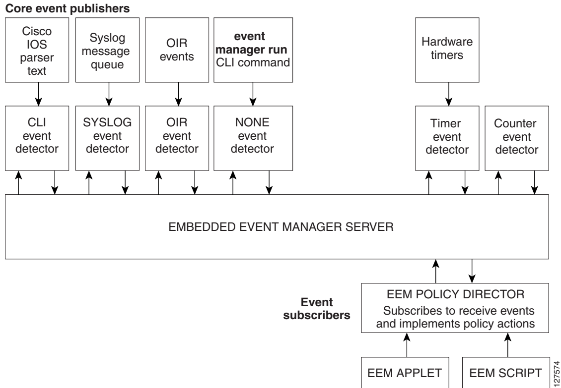
Figure 36-1 Embedded Event Manager Core Event Detectors
