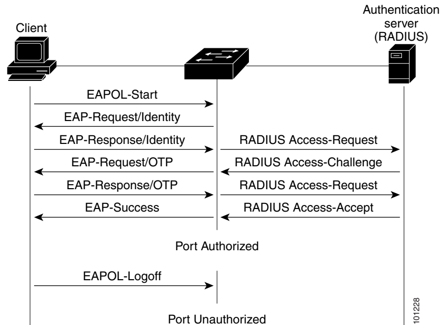
Figure 10-3 Message Exchange
