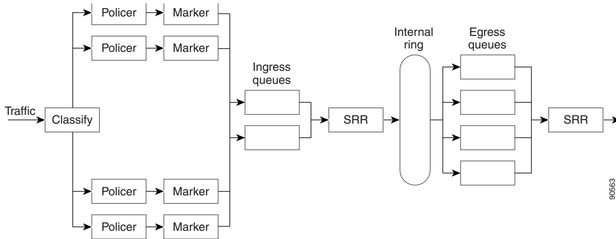
Figure 34-6 Ingress and Egress Queue Location
