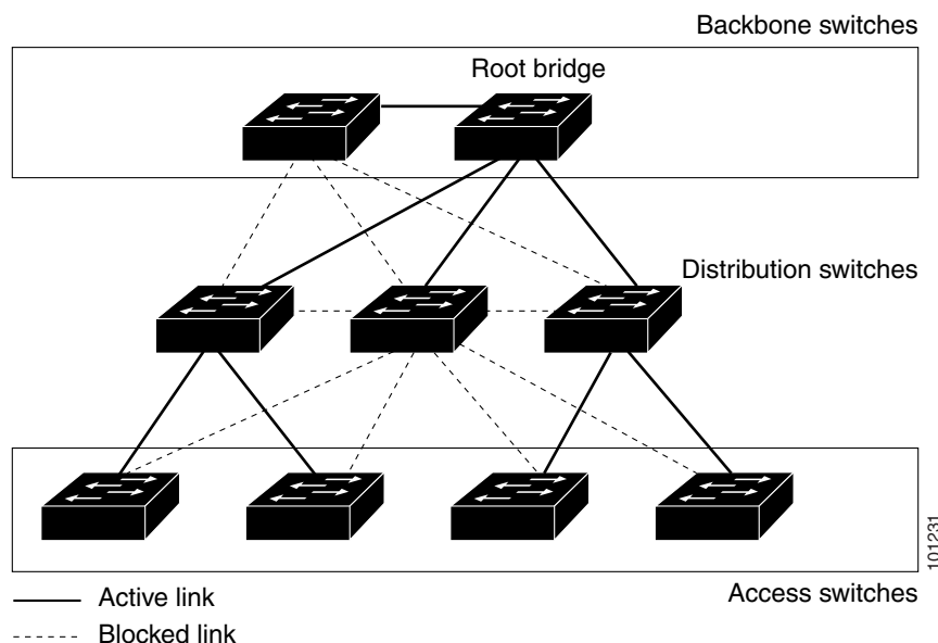
Figure 18-2 Switches in a Hierarchical Network
