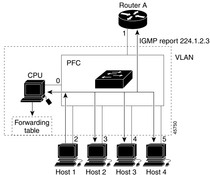
Figure 23-1 Initial IGMP Join Message
