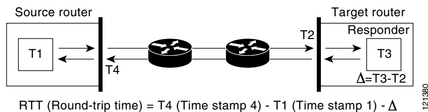
Figure 40-2 Cisco IOS IP SLAs Responder Time Stamping
