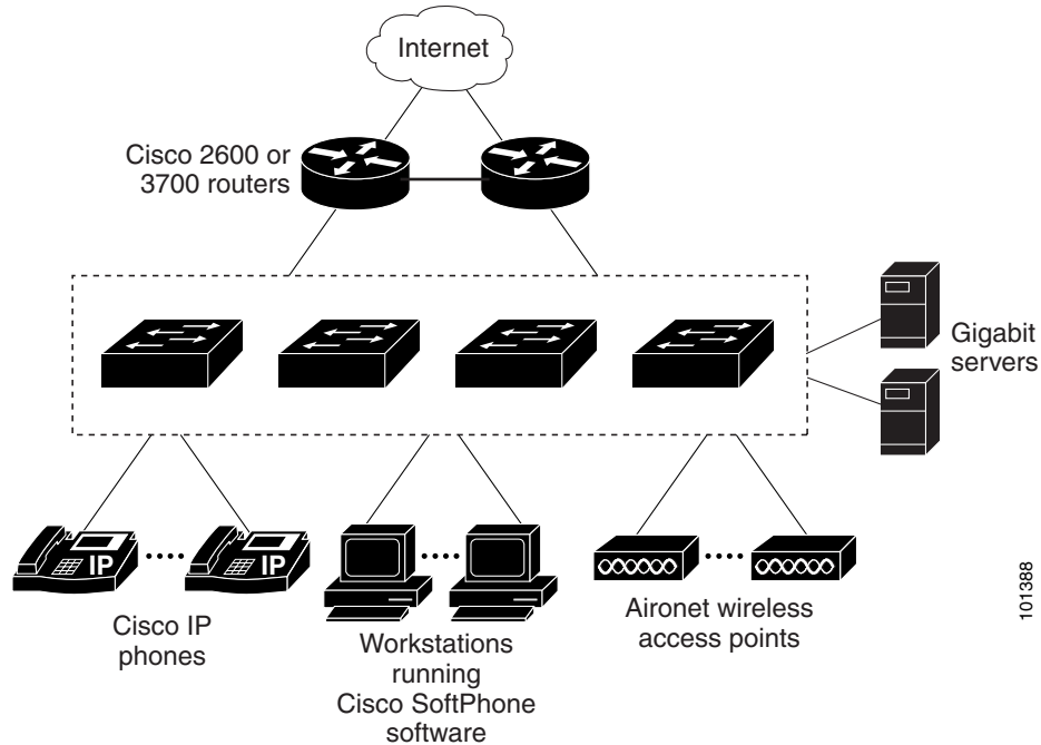
Figure 0-3 Catalyst 3560 Switches in a Collapsed Backbone Configuration
