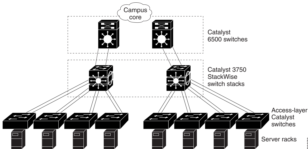
Figure 0-2 Server Aggregation
