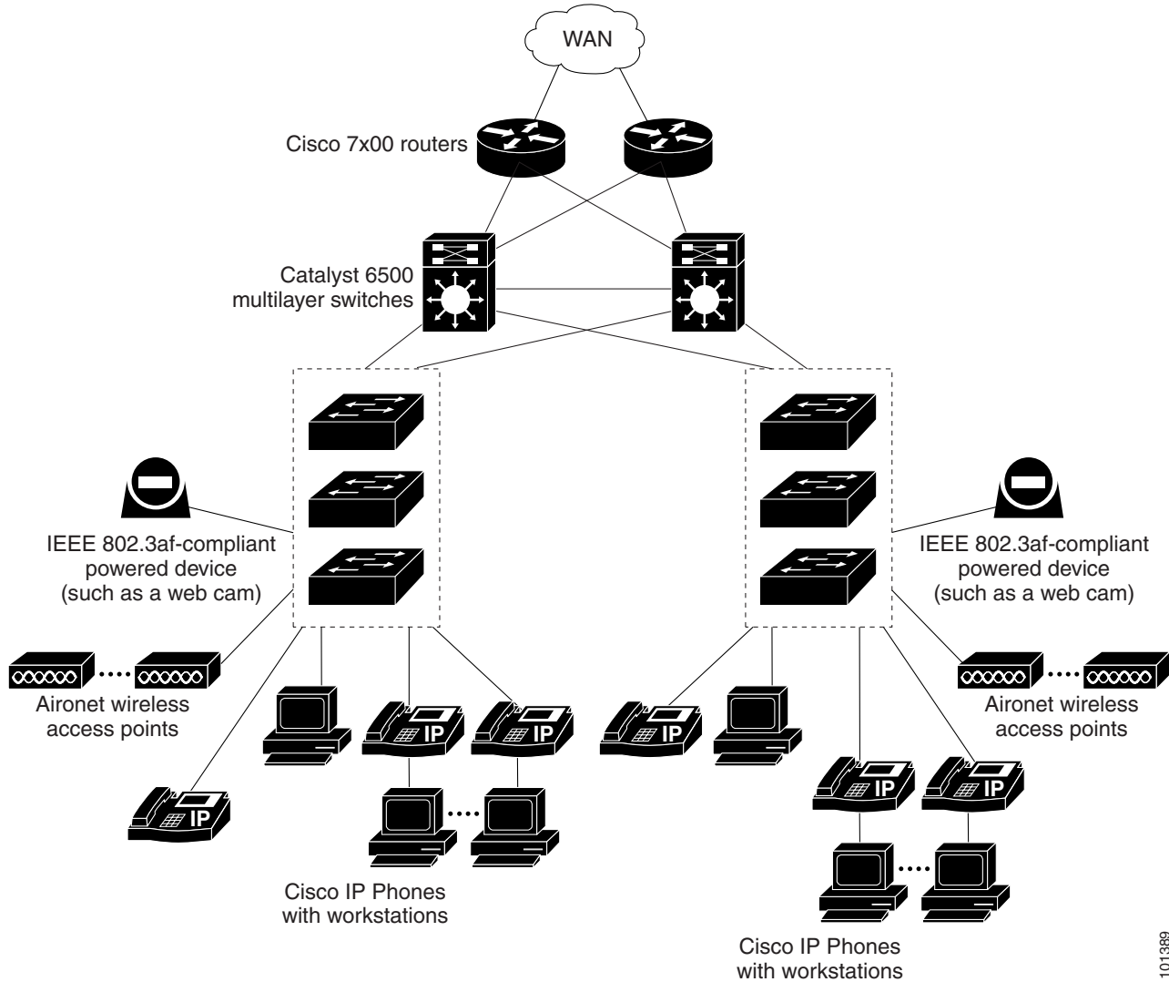
Figure 0-4 Catalyst 3560 Switches in Wiring Closets in a Backbone Configuration
