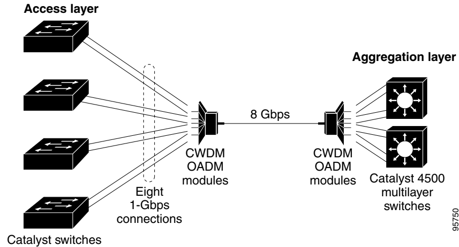
Figure 0-5 Long-Distance, High-Bandwidth Transport Configuration
