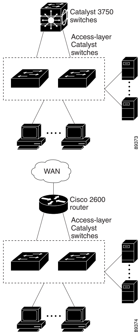
Figure 0-1 High-Performance Workgroup (Gigabit-to-the-Desktop)
