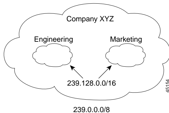
Figure 41-6 Administratively-Scoped Boundaries
