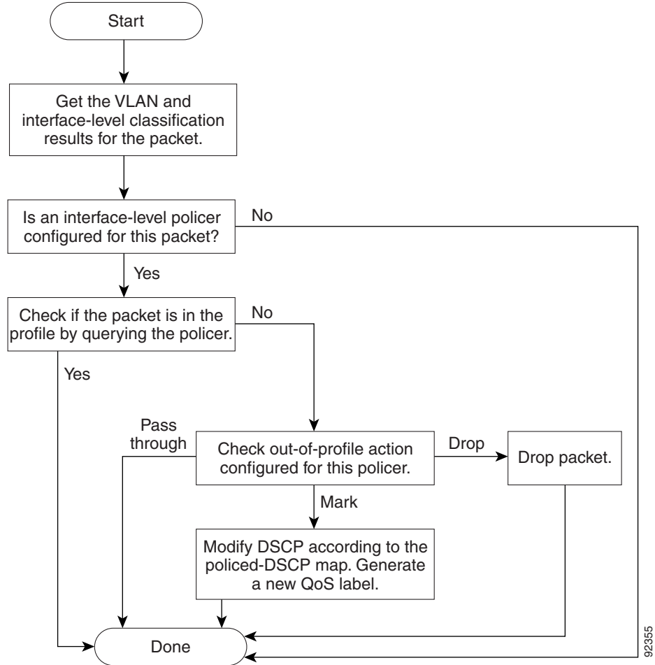
Figure 32-5 Policing and Marking Flowchart on SVIs
