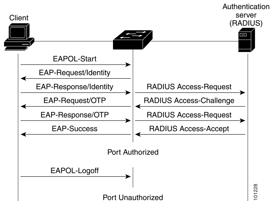
Figure 9-2 Message Exchange
