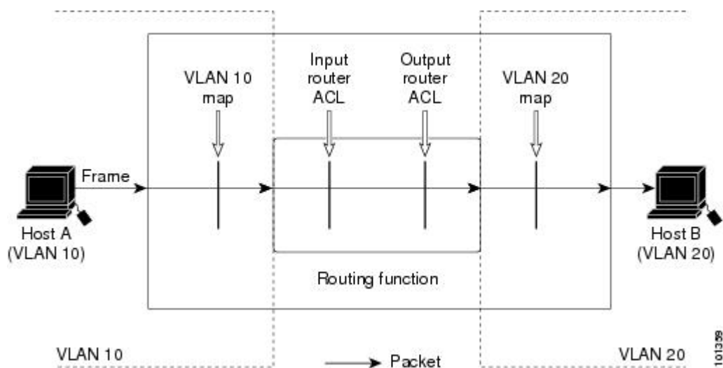
Figure 6: Applying ACLs on Routed Packets
