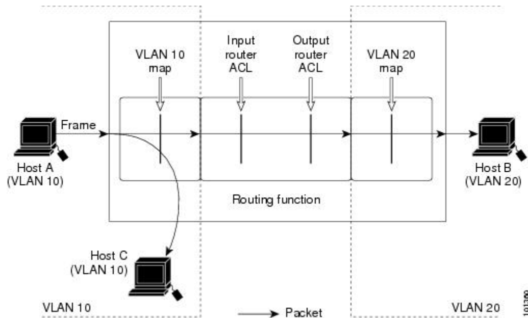
Figure 7: Applying ACLs on Multicast Packets
