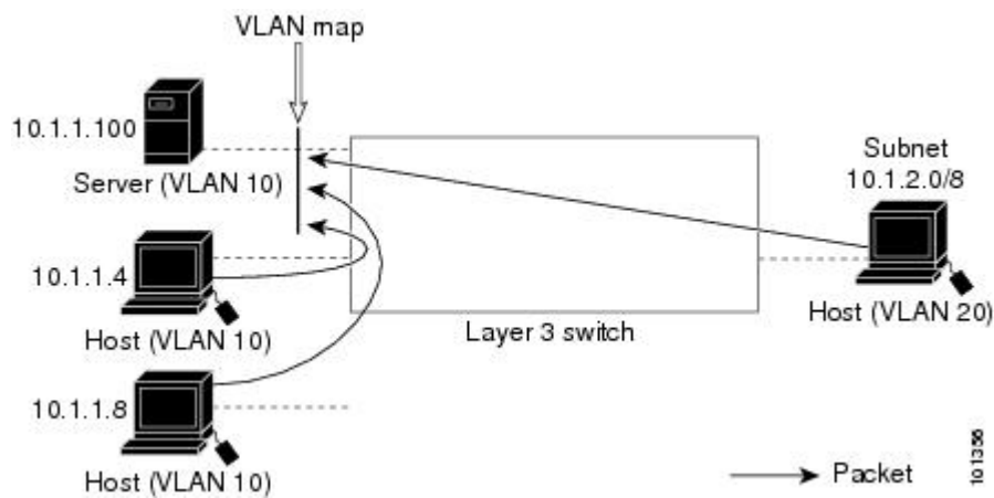
Figure 3: Restricting Access to a Server on Another VLAN
