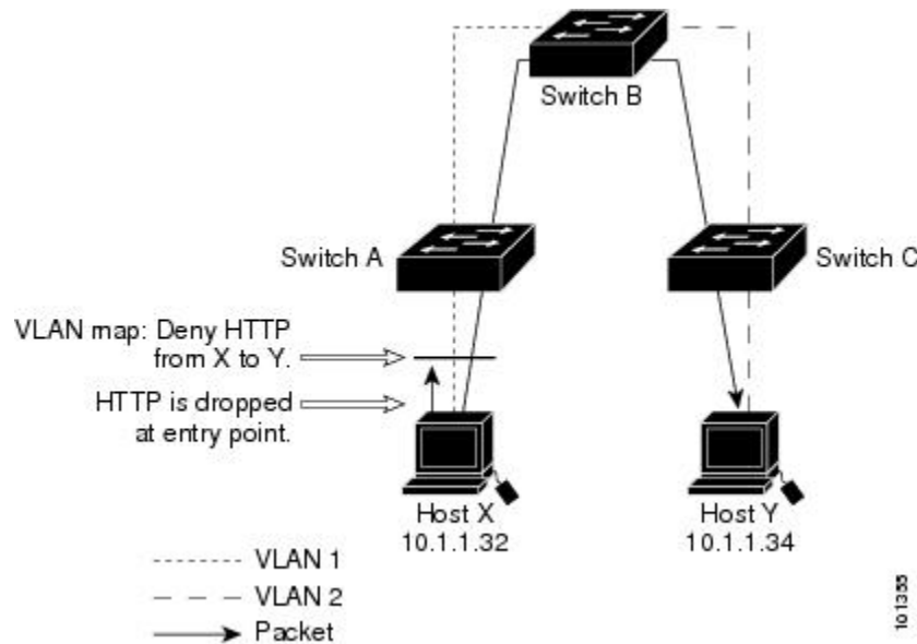
Figure 2: Wiring Closet Configuration
