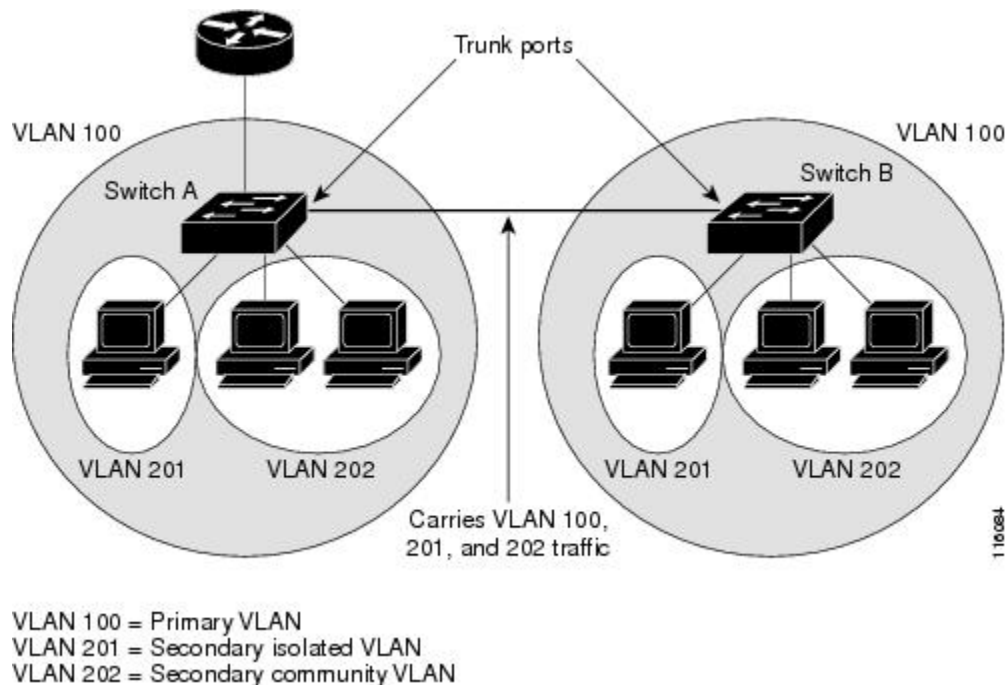
Figure 2: Private VLANs Across Switches
