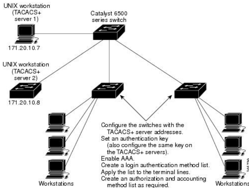
Figure 1: Typical TACACS+ Network Configuration
