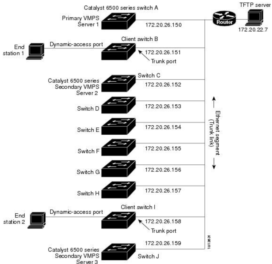
Figure 1: Dynamic Port VLAN Membership Configuration
