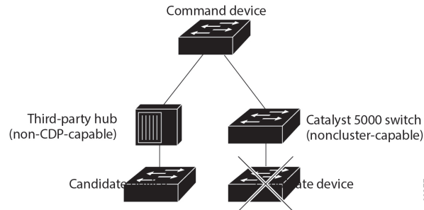
Figure 2: Discovery Through Non-CDP-Capable and Noncluster-Capable Devices
