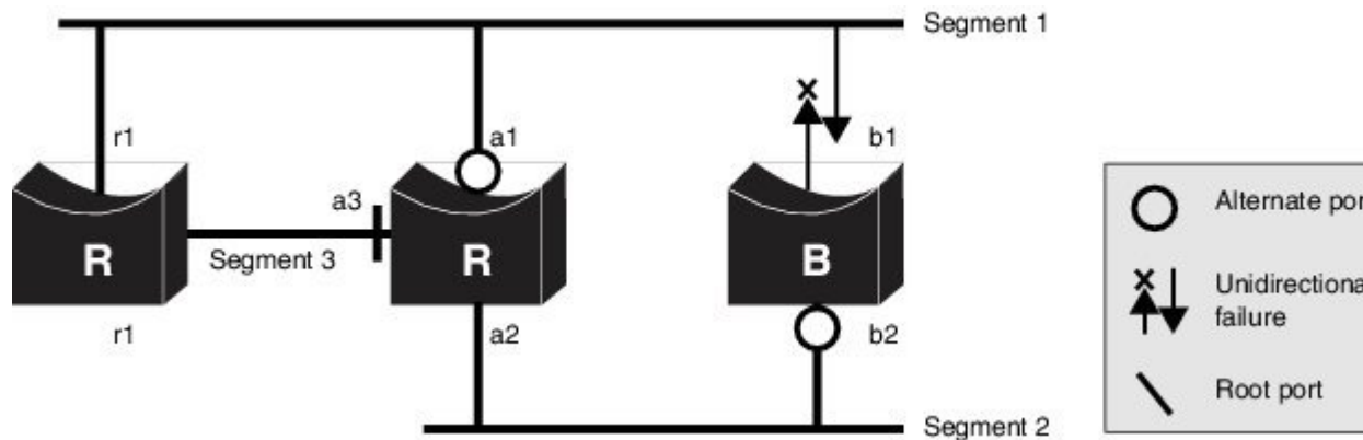
Figure 8: Bridging Loops on Shared Segments
