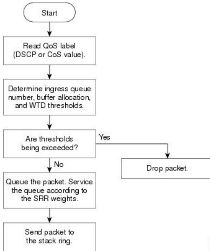
Figure 7: Queueing and Scheduling Flowchart for Ingress Ports on the Switch
