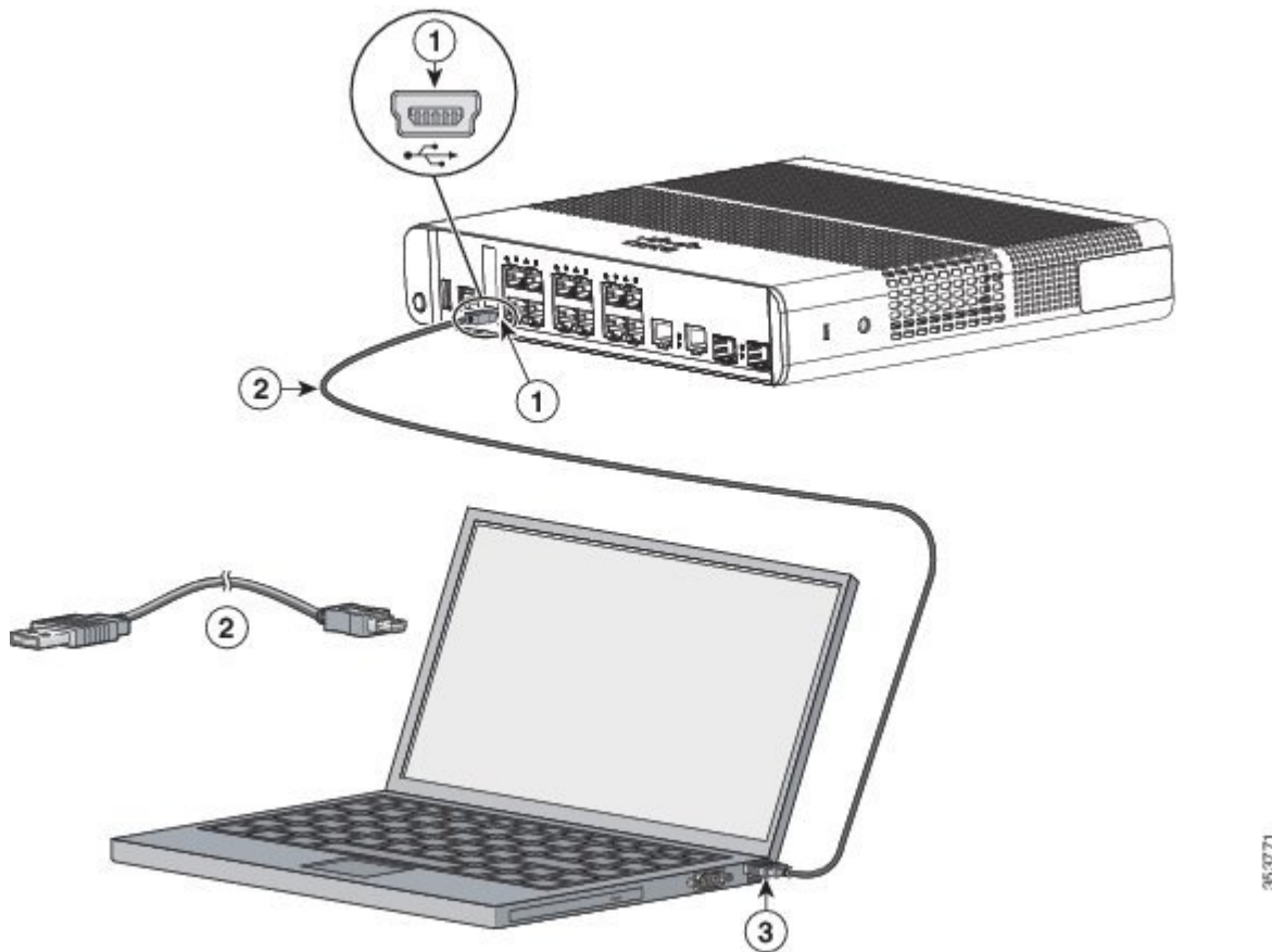
Figure 1: Connecting the USB Console Cable to the Switch
