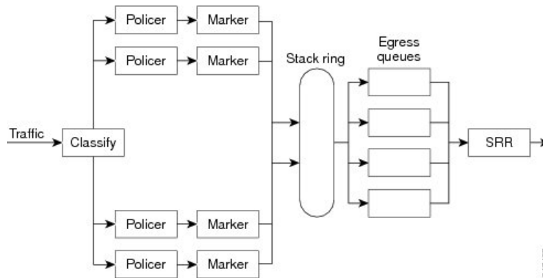
Figure 5: Ingress and Egress Queue Location on Switch
