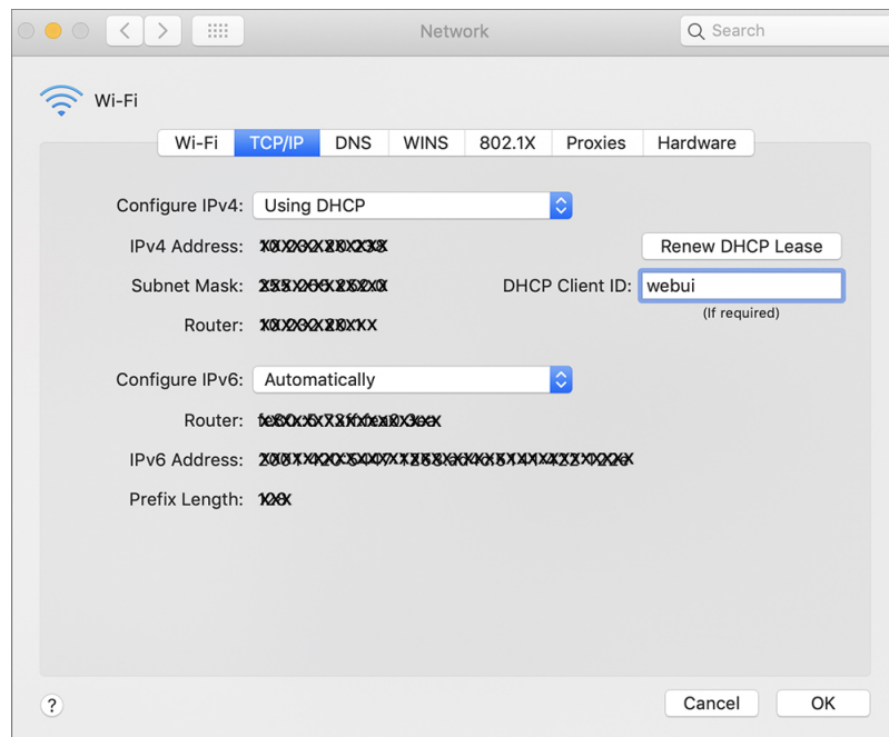
Figure 2: Setting up DHCP Client Identifier on MAC
