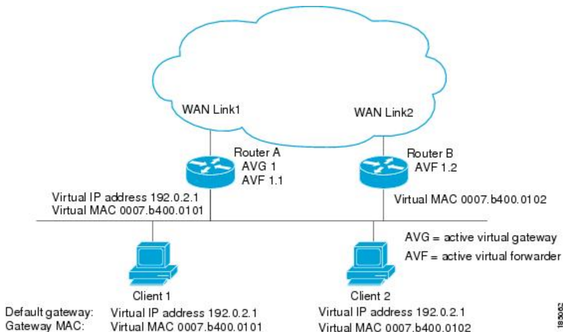
Figure 1: GLBP Topology
