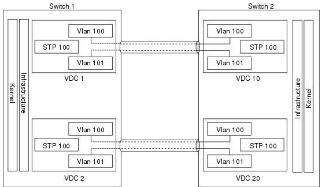
Figure 1: VDCs with Layer 2 Services
