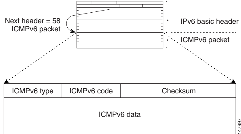
Figure 44-6 IPv6 ICMP Packet Header Format
