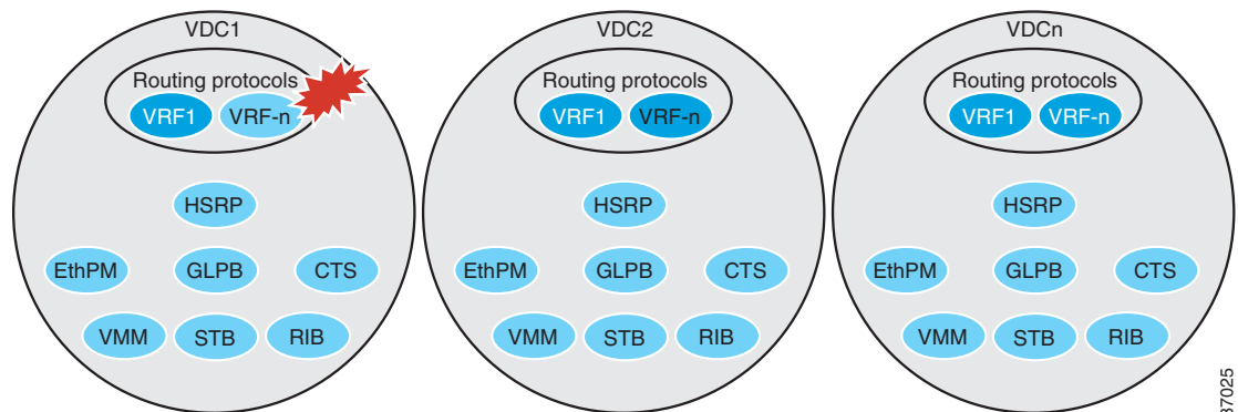
Figure 1-8 Fault Isolation within VDCs
