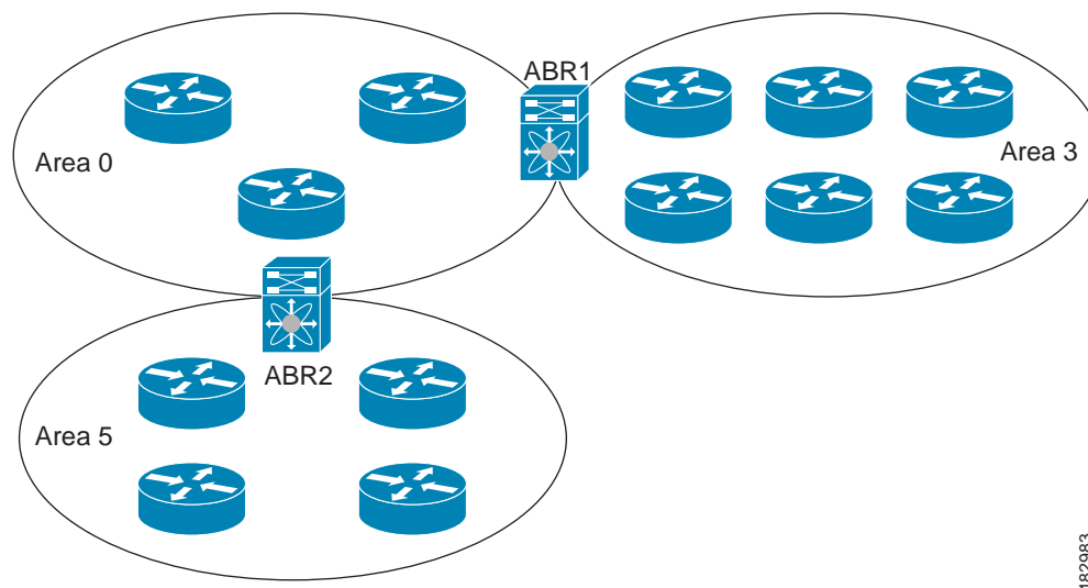
Figure 7-2 OSPFv3 Areas
