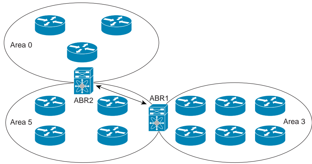
Figure 7-4 Virtual Links
