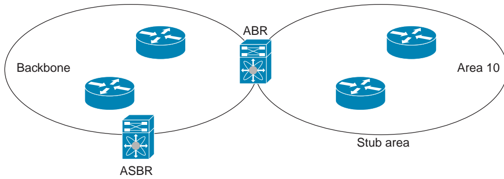
Figure 7-3 Stub Area
