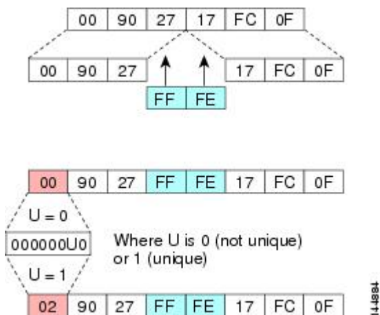
Figure 2: Interface Identifier Format
