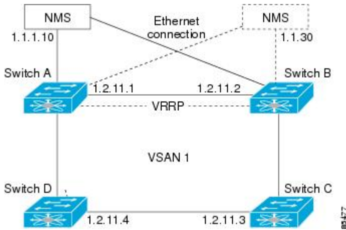
Figure 3: VRRP Functionality
