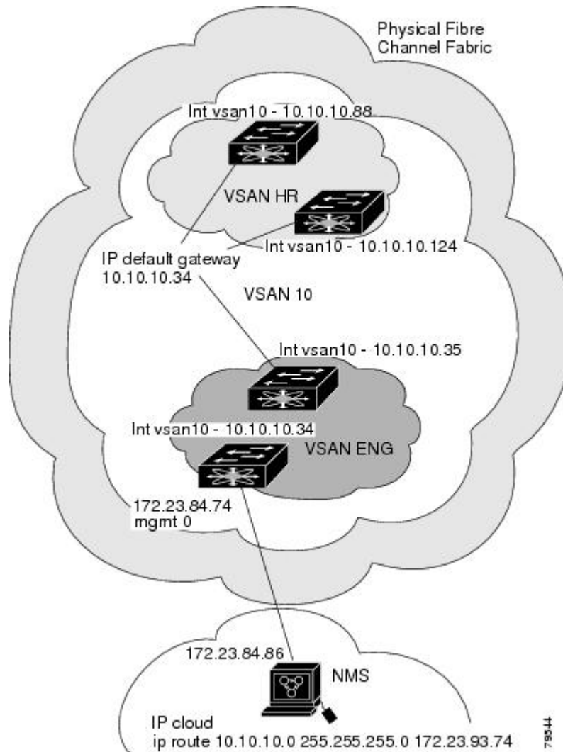
Figure 5: Overlay VSAN Configuration Example
