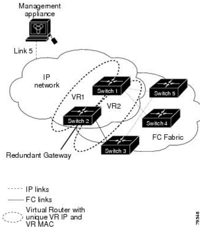
Figure 4: Redundant Gateway
