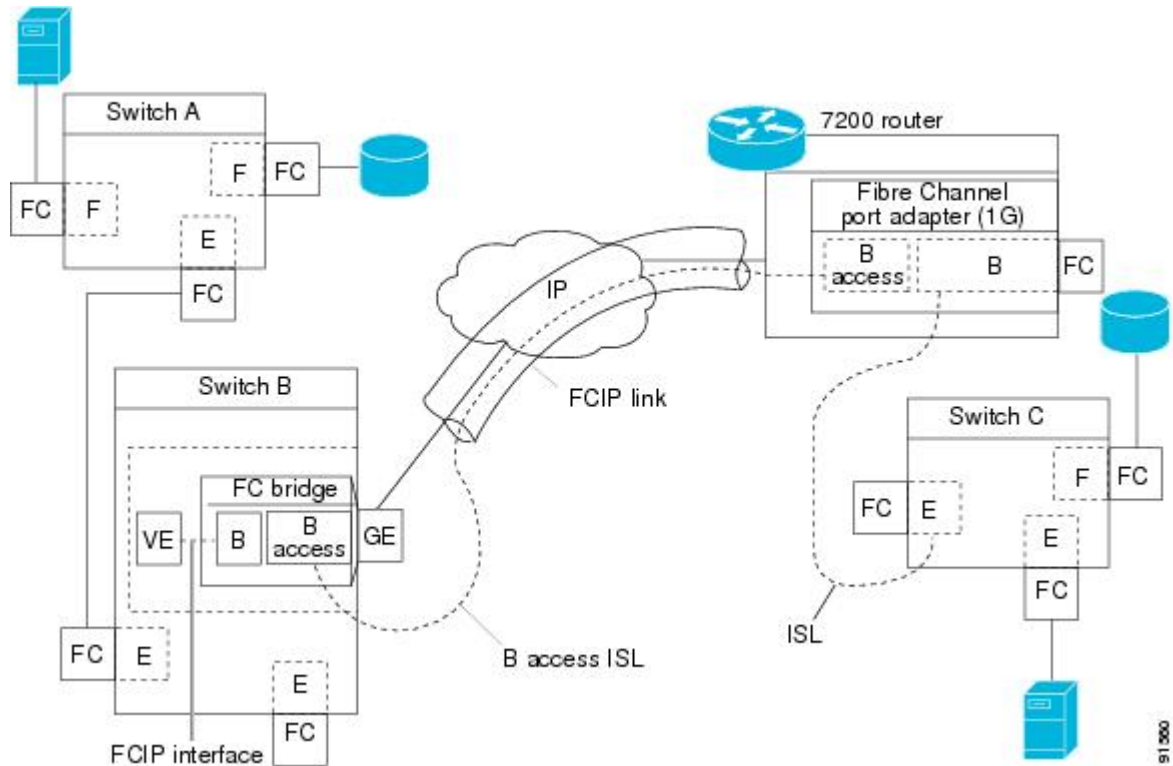
Figure 11: FCIP Link Terminating in a B Port Mode
