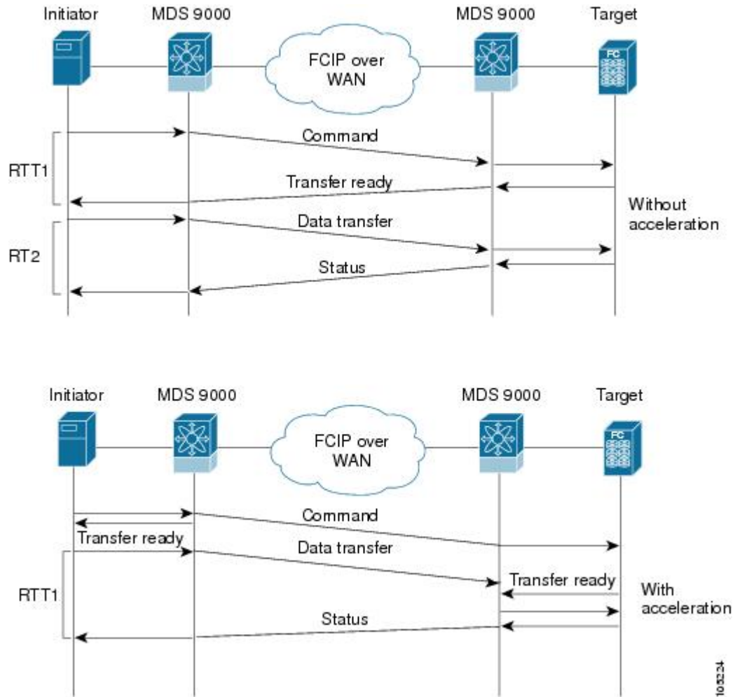
Figure 12: FCIP Link Write Acceleration
