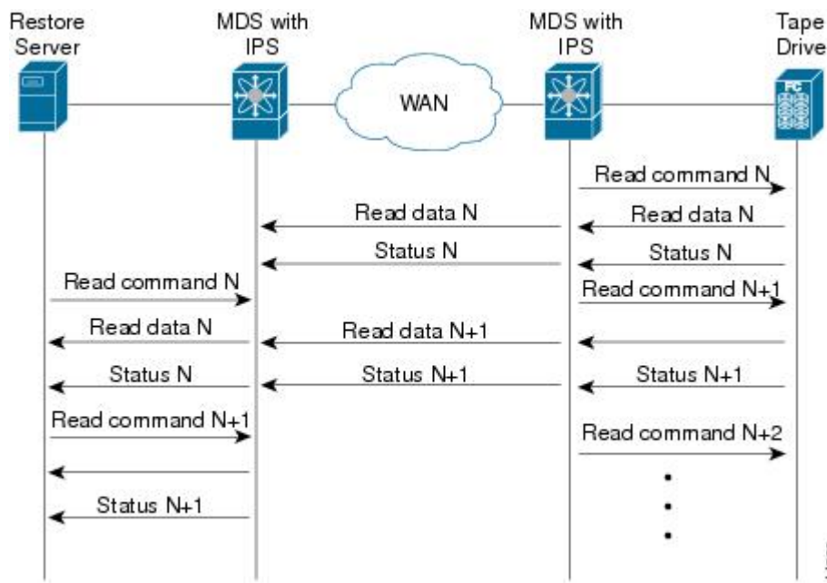
Figure 14: FCIP Link Tape Acceleration for Read Operations
