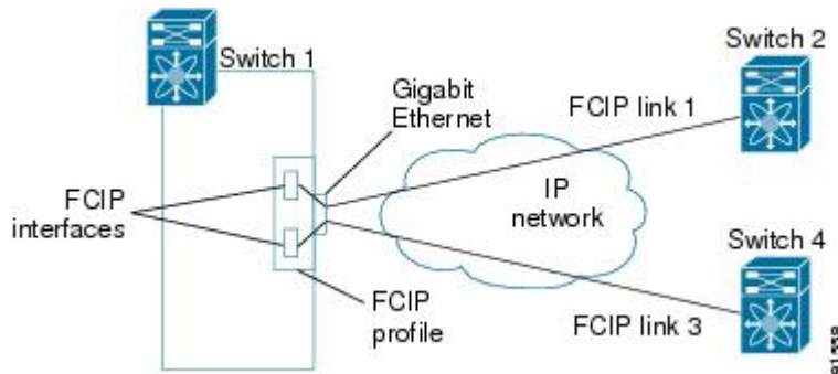
Figure 4: FCIP Profile and FCIP Links
