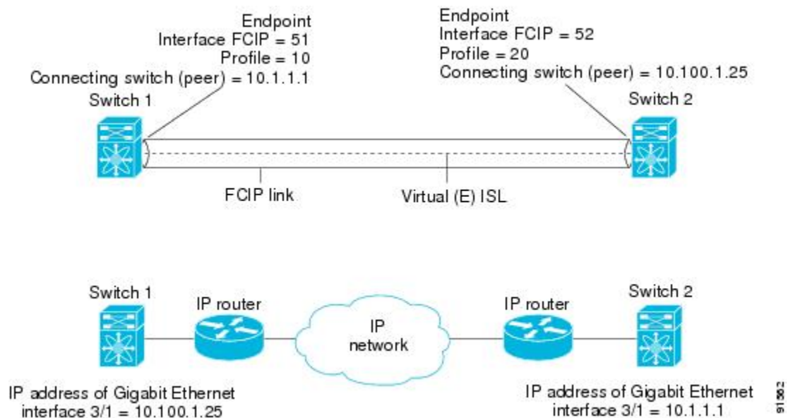
Figure 3: Assigning Profiles to Each Gigabit Ethernet Interface
