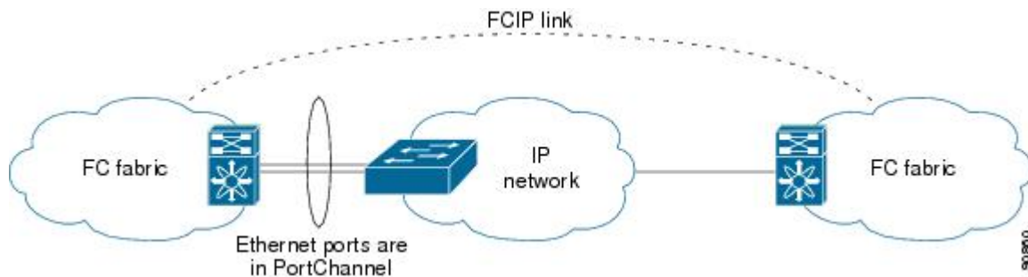
Figure 9: Ethernet PortChannel-Based High Availability
