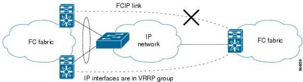
Figure 8: VRRP-Based High Availability
