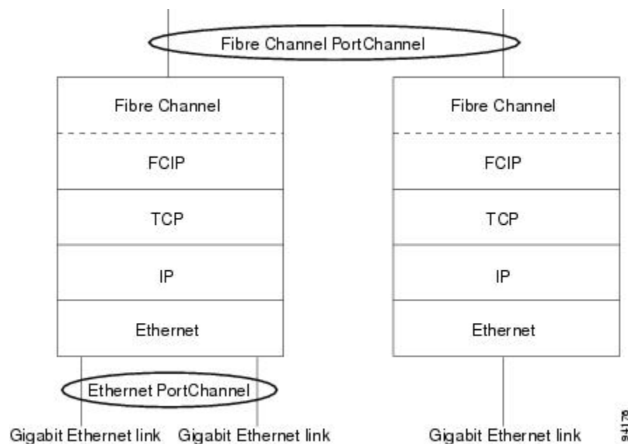
Figure 10: PortChannels at the Fibre Channel and Ethernet Levels
