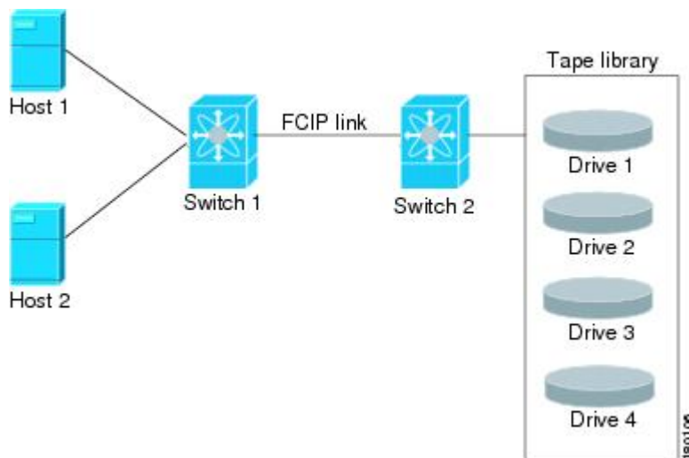
Figure 15: FCIP LUN Mapping Example
