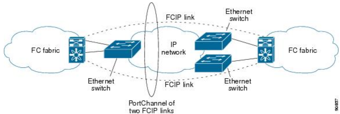
Figure 6: PortChannel-Based Load Balancing
