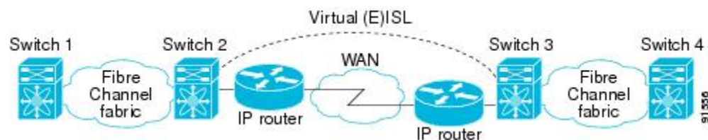
Figure 1: Fibre Channel SANs Connected by FCIP
