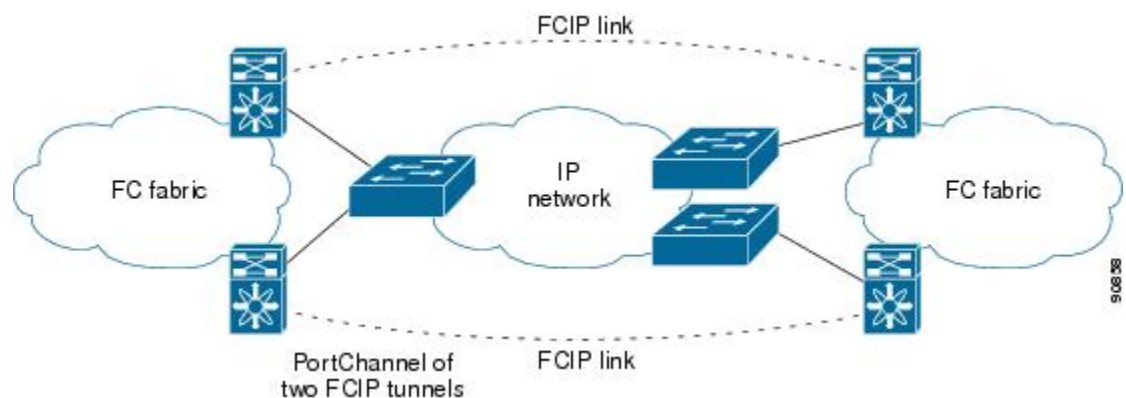
Figure 7: FSPF-Based Load Balancing
