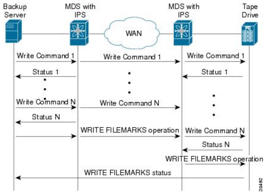
Figure 13: FCIP Link Tape Acceleration for Write Operations
