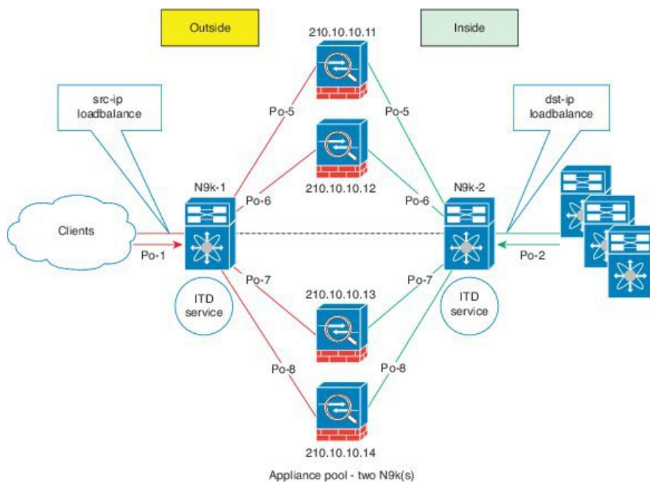
Figure 15: Sandwich Deployment Mode
