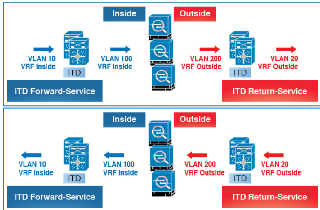
Figure 19: ITD ASA Deployment
