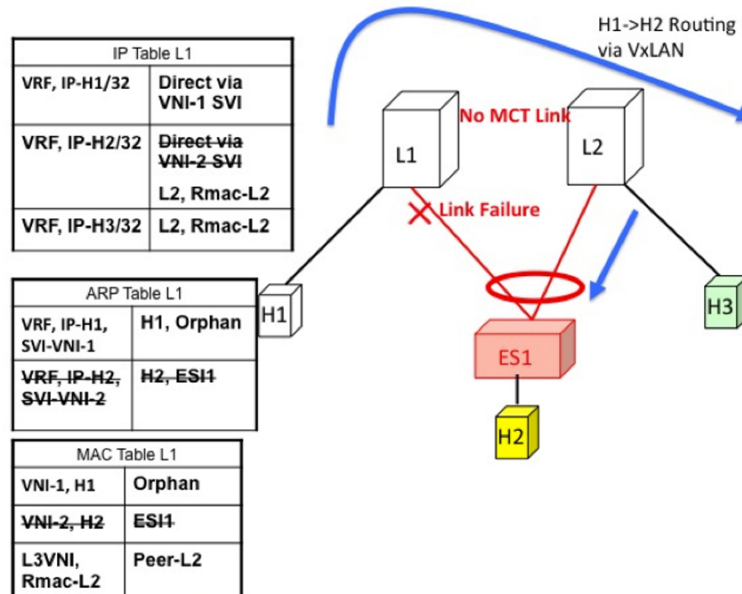
Figure 5: H1, H2, and H3 are in different VLANs. ESI fails on L1. H1->H2 routing happens via VXLAN tunnel encapsulation.
