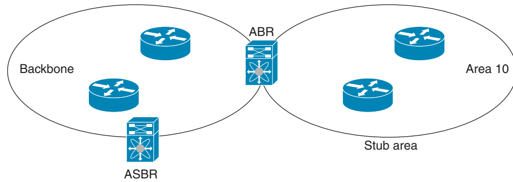
Figure 5-3 Stub Area
