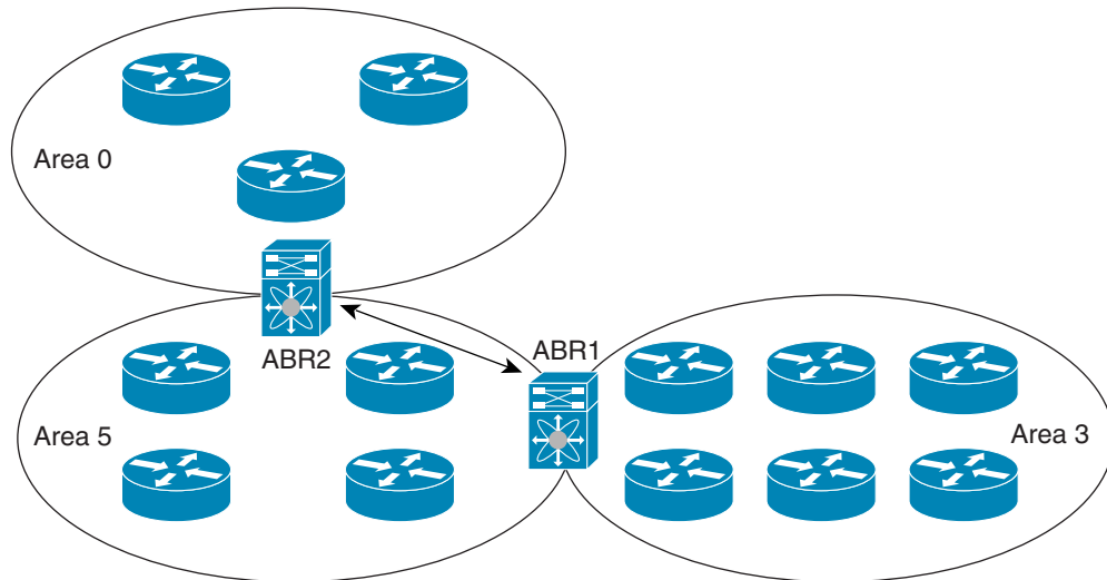
Figure 5-4 Virtual Links
