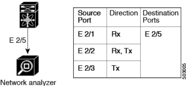
Figure 1: SPAN Configuration
