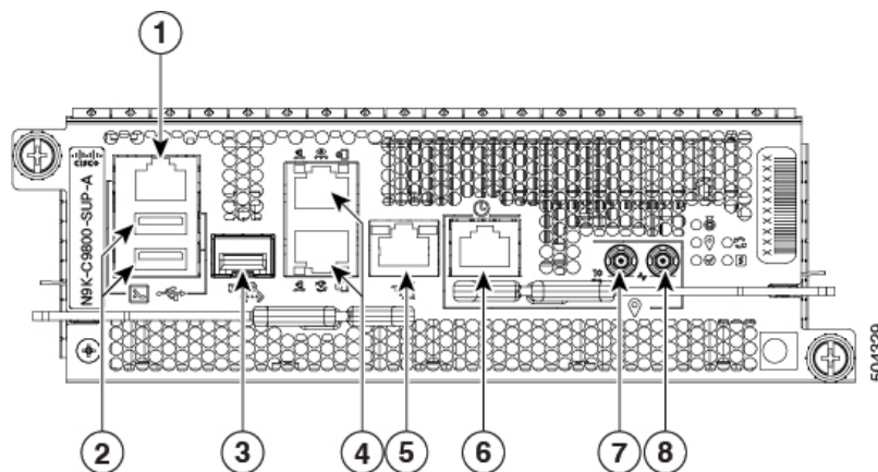
Figure 1: Supervisor Module
