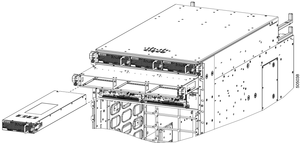
Figure 15: HV Power Supply Trays
