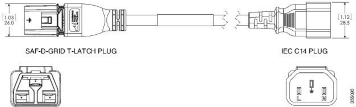
Figure 16: SAF-D-Grid Plug
