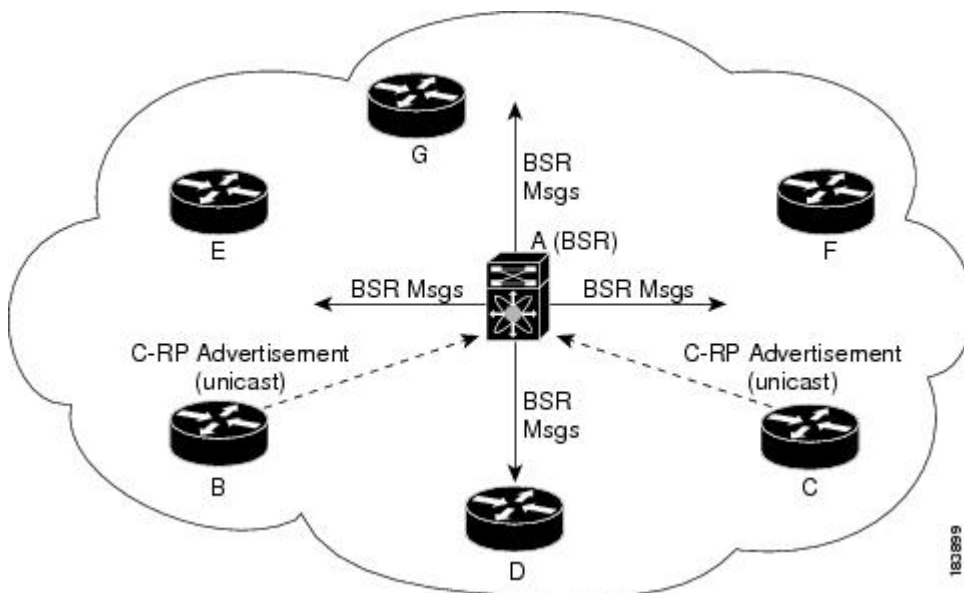
Figure 1: BSR Mechanism
